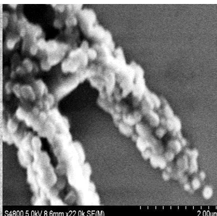
Figure 3. SEM image of C_{60/70} clusters synthesized by thermal evaporation of xylene from the volume of single drop of C_{60/70} solution at \sim 28^\circ\text{C} .
