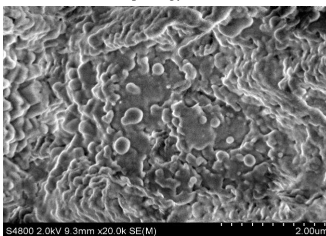
Figure 4. SEM-image of nanostructured coating consists of C_{60/70} clusters synthesized by thermal evaporation of xylene from the volume of drying drop of fullerene solution. The substrate temperature was \sim 30^\circ\text{C} . The initial fullerene concentration in the solution is \sim 2.6\cdot 10^{-4} \text{ mol}\cdot\text{L}^{-1} .
