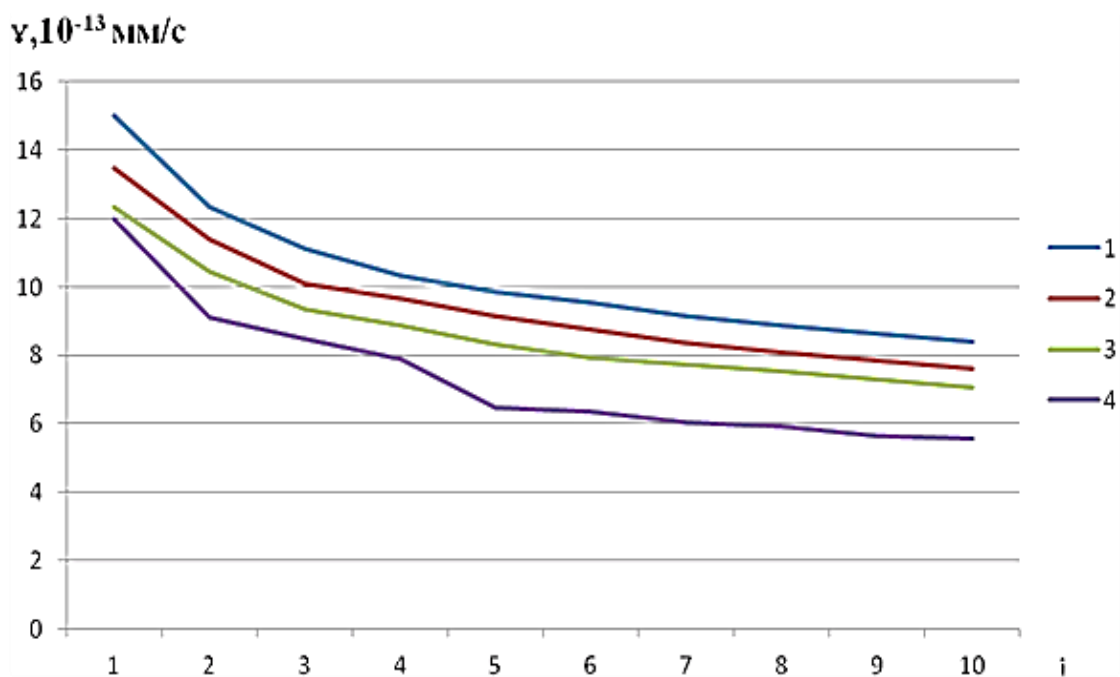
Figure 1. The speed of eating the wheel teeth depends on the number of contact surfaces: 1 - q=100 N/mm; 2 - q= 200 N/mm; 3 - q=300 N/mm; 4 - q=400 N/mm;
