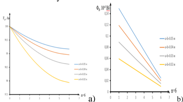
Fig. The graphs of change flux and m.m.f. on longitudinal sections of transformation signal of circuit of intelligent sensors and measurement systems where:
